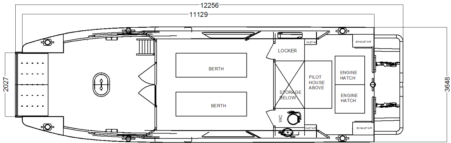
DECK PLAN
