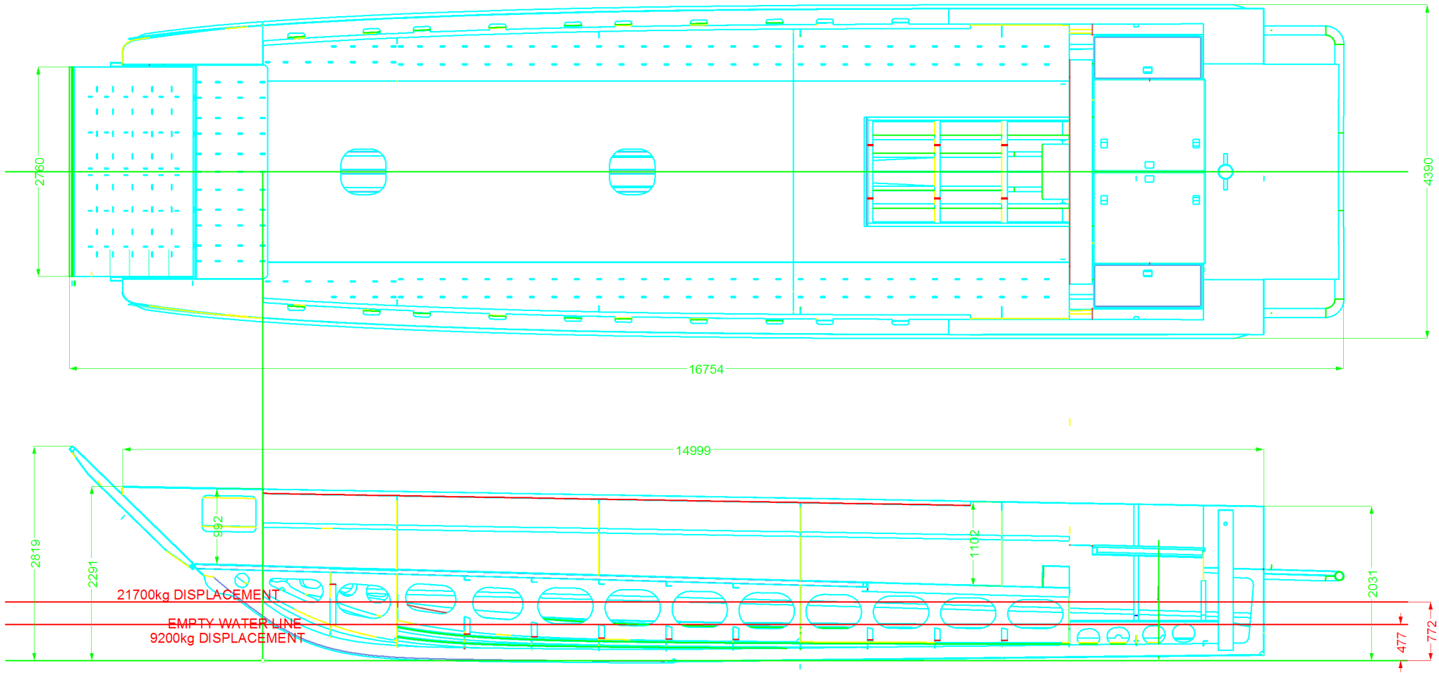
15 X 4.4 METER LANDING CRAFT(PRELIMINARY) 2/7/05
