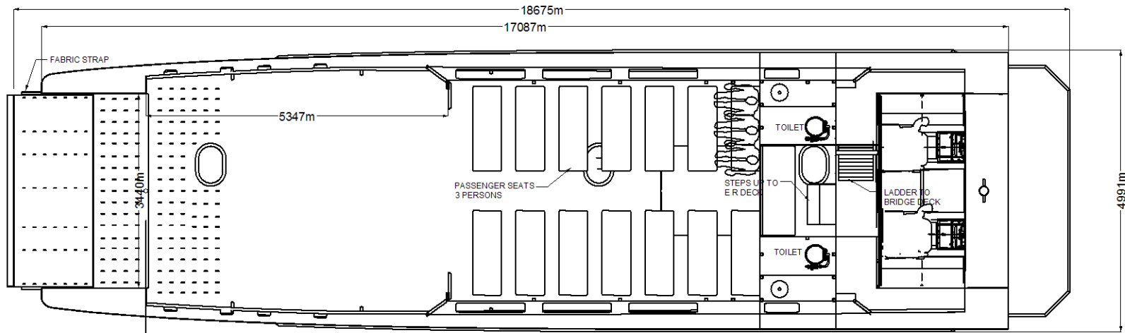
DECK PLAN
