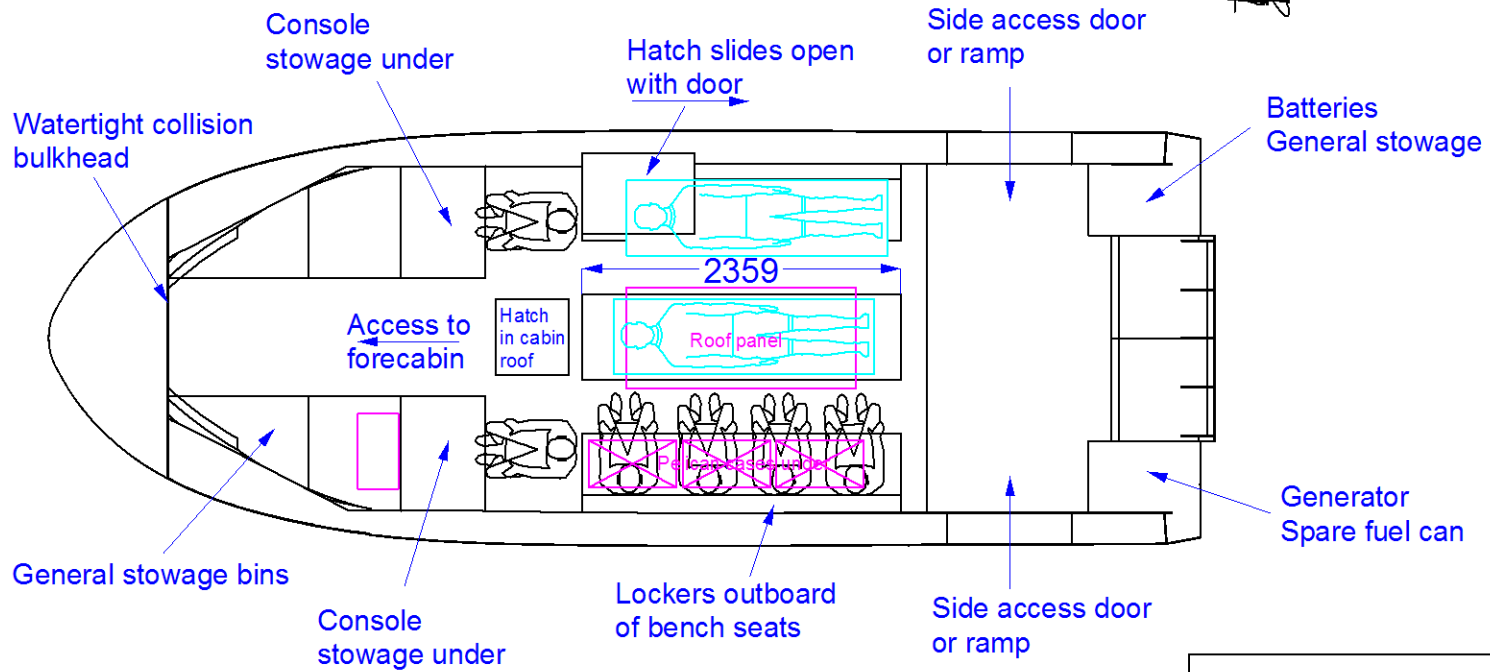
RESCUE EAGLE 8.5m Water ambulance
