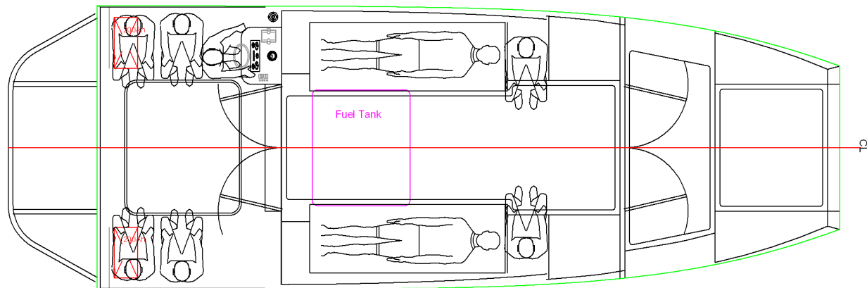
Deck Layout
