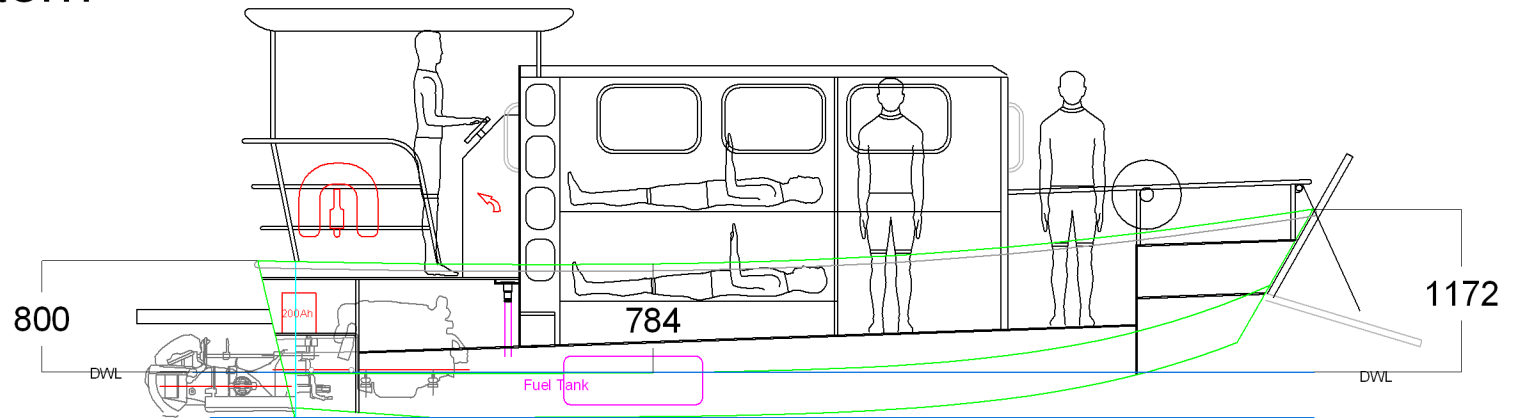
Side Elevation
